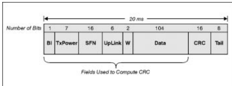
Figure 5-1 Perch1(BCCH) Frame
