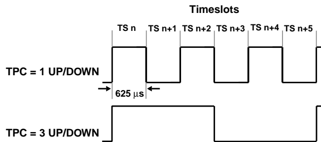
Figure 3-8 Example TPC Output Waveform
