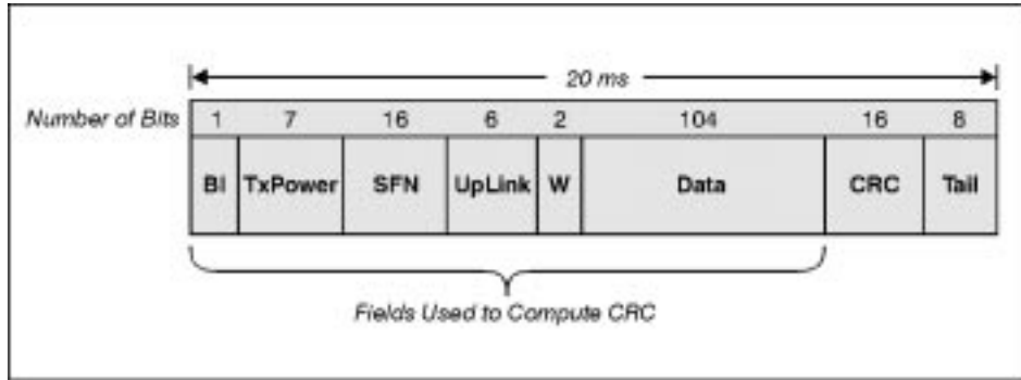
Figure 4-1 Perch1(BCCH) Frame
